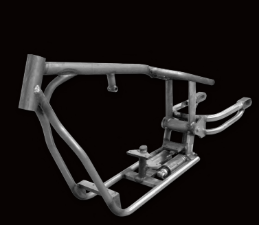
WISHBONE / SOFTAIL
