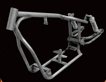
WISHBONE / SWINGARM
